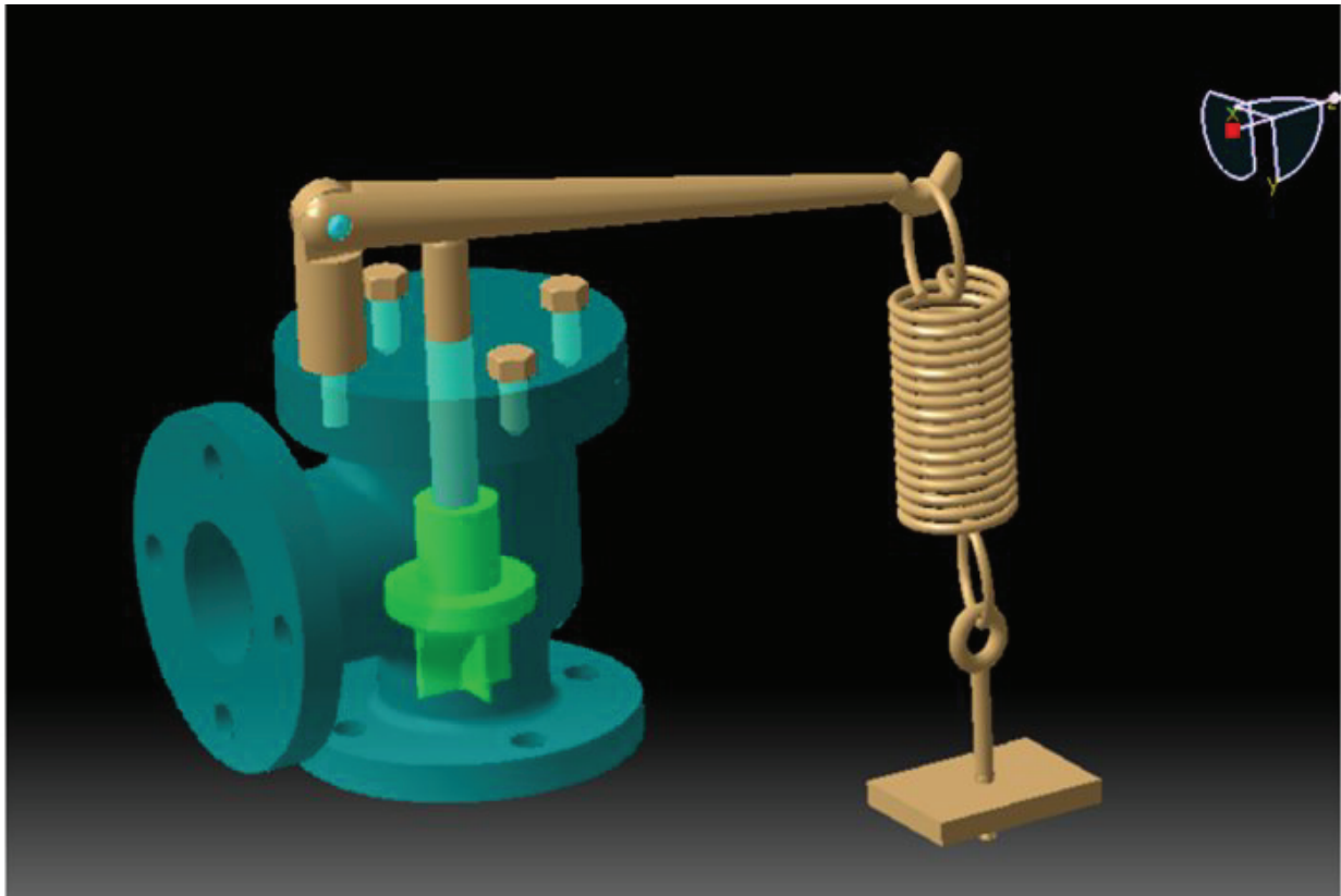
Fig. 18.37A Spring loaded relief valve
