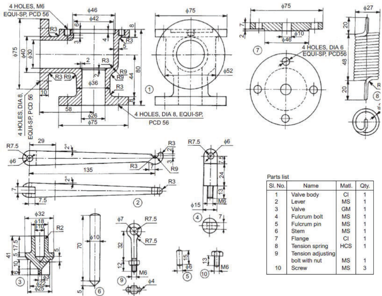
Fig. 18.37 Spring loaded relief valve
