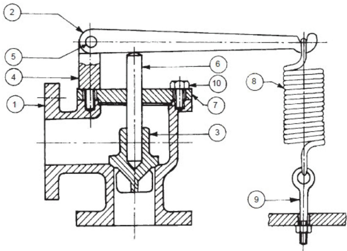
Fig. 18.37A Spring loaded relief valve
